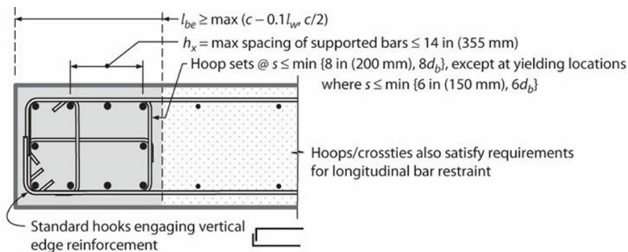
(b) Ordinary boundary element where \rho_{be} > 400/f_{yr} psi (2.8/ f_{yr} MPa)
